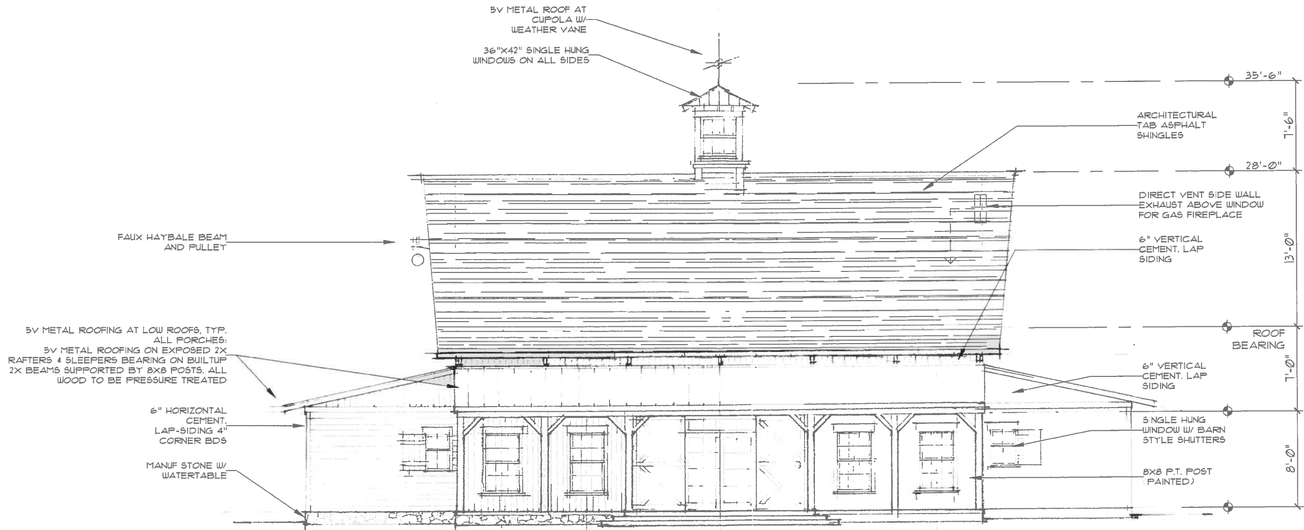
FRONT ELEVATION - (REAR ELEVATION SIMILAR)
